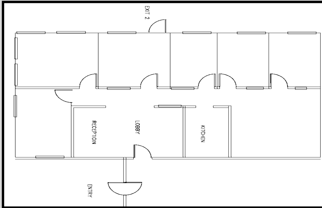
GROUND FLOOR OFFICE LAY-OUT
